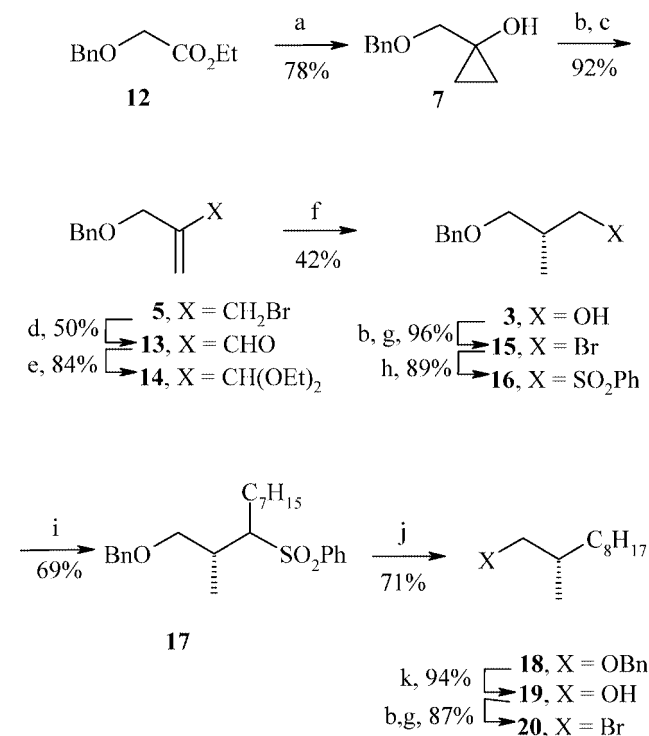
Scheme 3. Synthesis of bromide 20 . Reagents and conditions: (a) \text{EtMgBr} , \text{Ti}(\text{O}i\text{Pr})_4 ; (b) \text{MsCl} , \text{Et}_3\text{N} ; (c) \text{MgBr}_2 ; (d) \text{DMSO} , \text{NaHCO}_3 ; (e) \text{HC}(\text{OEt})_3 , \text{H}^+ ; (f) baker's yeast; (g) \text{Bu}_4\text{NBr} ; (h) \text{Bu}_4\text{NPhSO}_2 ; (i) 1. \text{BuLi} ; 2. \text{C}_7\text{H}_{15}\text{I} ; (j) \text{Na}/\text{Hg} , \text{EtOH} ; (k) \text{H}_2 , \text{Pd}/\text{C} .
