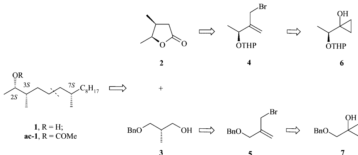
Scheme 1. Retrosynthetic analysis of 1 and ac-1 .
