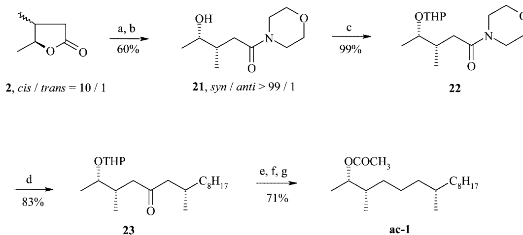
Scheme 4. Synthesis of 1 and ac-1 . Reagents and conditions: (a) morpholine, 100 °C, 24 h; (b) recrystallization from diethyl ether; (c) DHP, PPTS, CH 2 Cl 2 ; (d) (2 R )-2-methyldecyllithium, Et 2 O/THF, −78 °C; (e) N 2 H 4 , KOH, triethylene glycol, 180–210 °C; (f) MeOH, PPTS, reflux; (g) CH 3 COCl, Et 3 N, Et 2 O.
