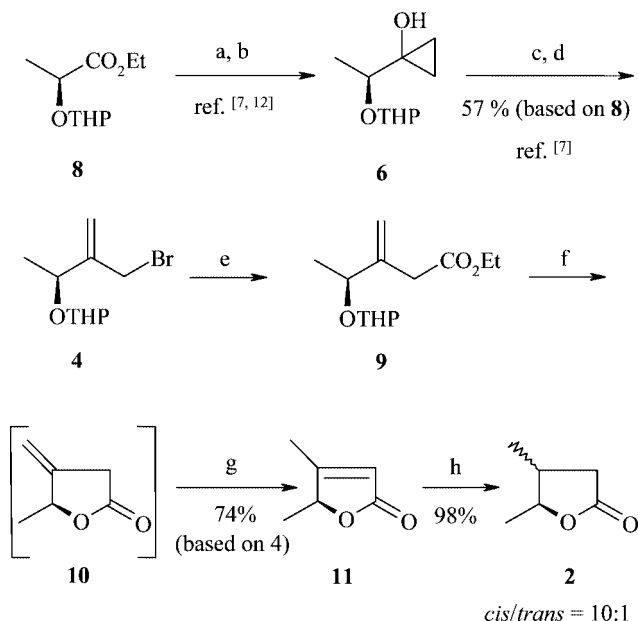
Scheme 2. Synthesis of lactone 2 . Reagents and conditions: (a) DHP, PPTS, \text{CH}_2\text{Cl}_2 , reflux; (b) \text{EtMgBr} , \text{Ti}(\text{O}i\text{Pr})_4 , \text{Et}_2\text{O}/\text{THF} ; (c) \text{MsCl} , \text{Et}_3\text{N} , \text{Et}_2\text{O} ; (d) \text{MgBr}_2 , \text{Et}_2\text{O}/\text{CHCl}_3 , reflux; (e) \text{Zn} , \text{CuCl} , 1,2-dibromoethane, \text{ClCO}_2\text{Et} , reflux; (f) \text{MeOH} , \text{THF} , \text{HCl} , reflux; (g) \text{Et}_3\text{N} , reflux; (h) \text{NaBH}_4 , \text{NiCl}_2 , \text{B}(\text{OH})_3 , \text{H}_2\text{O} .
